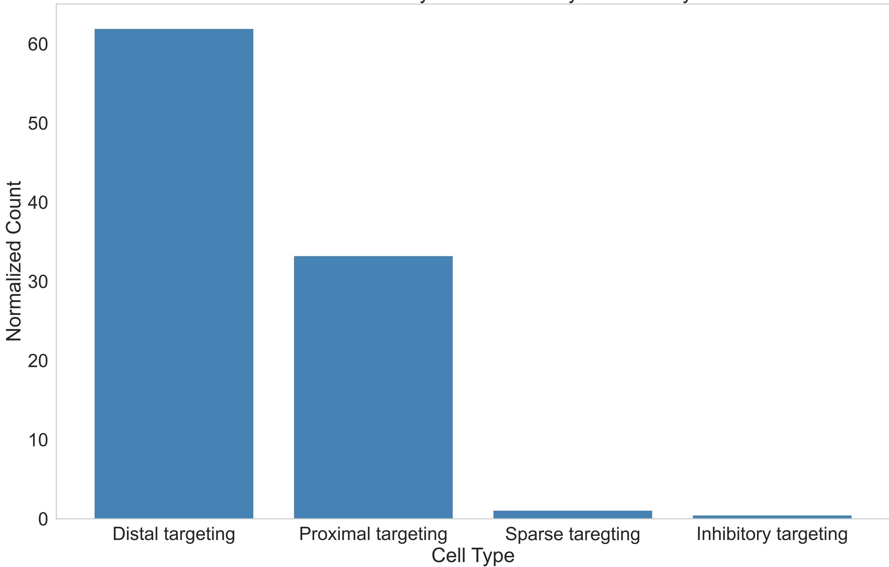
Outbound Inhibitory — No Assembly to Assembly
